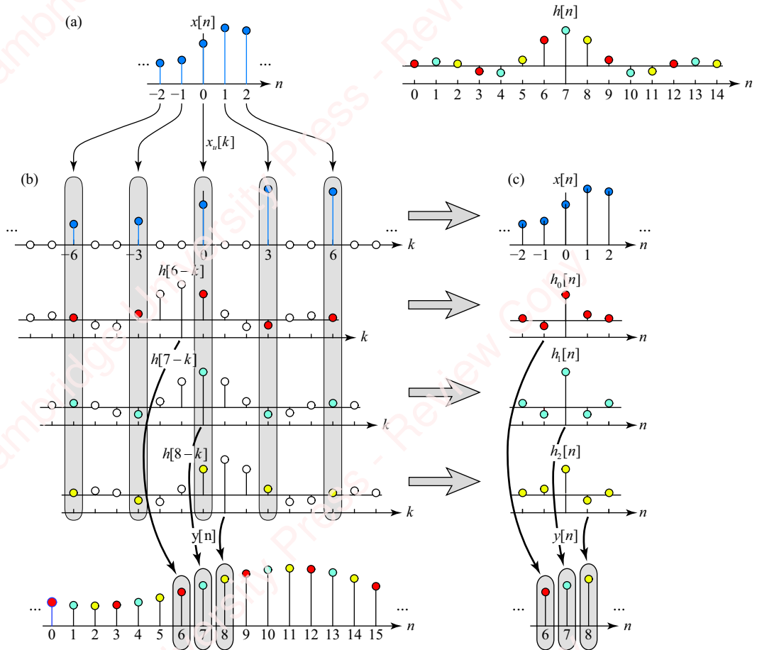
Figure 13.11 Polyphase upsampling
