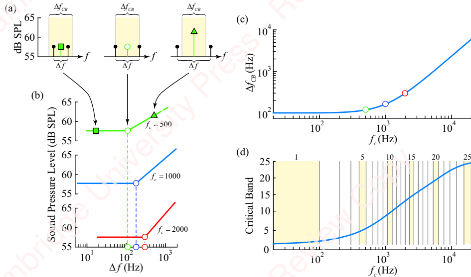
Figure 12.8 Critical bands
